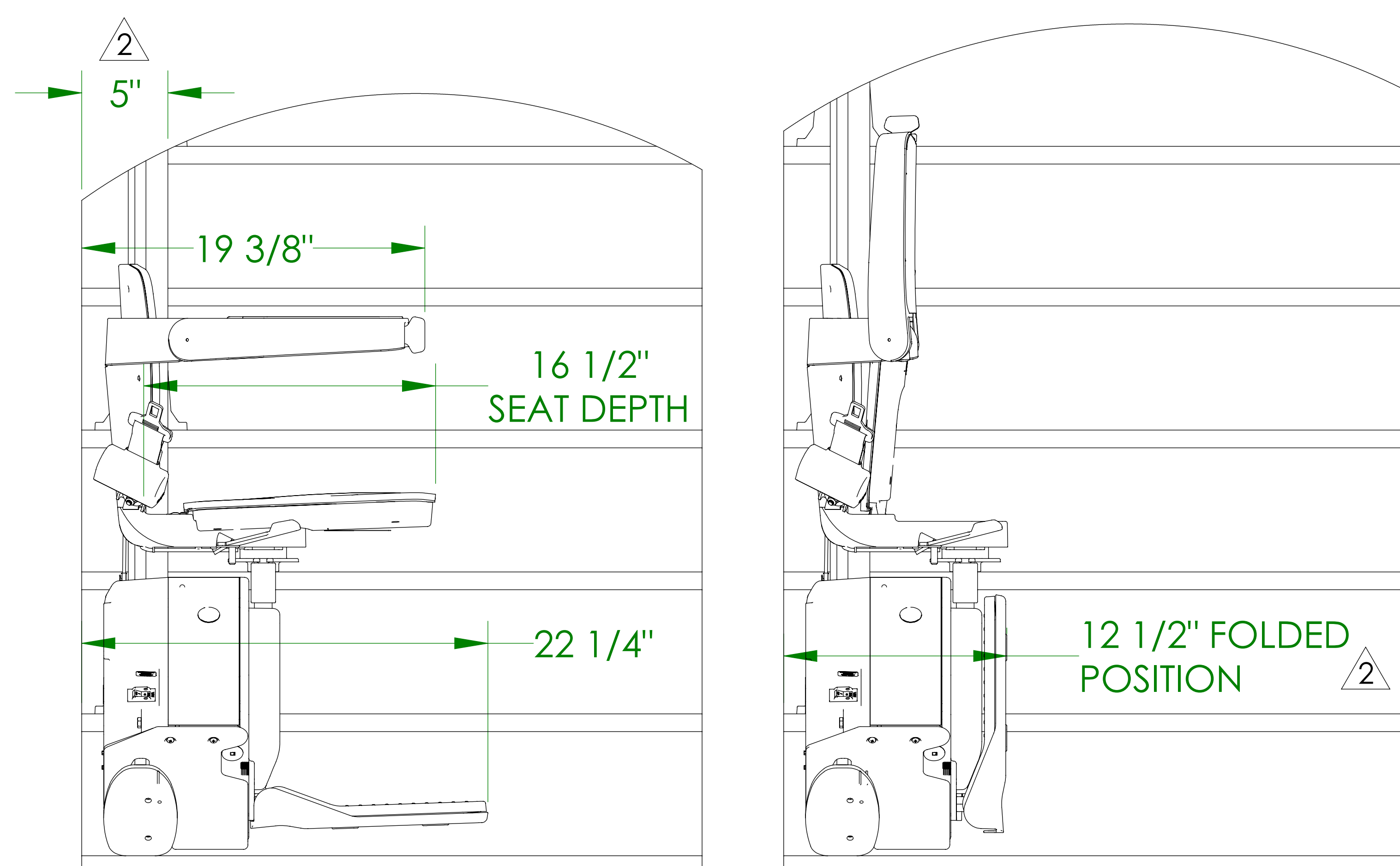
SIDE VIEWS
