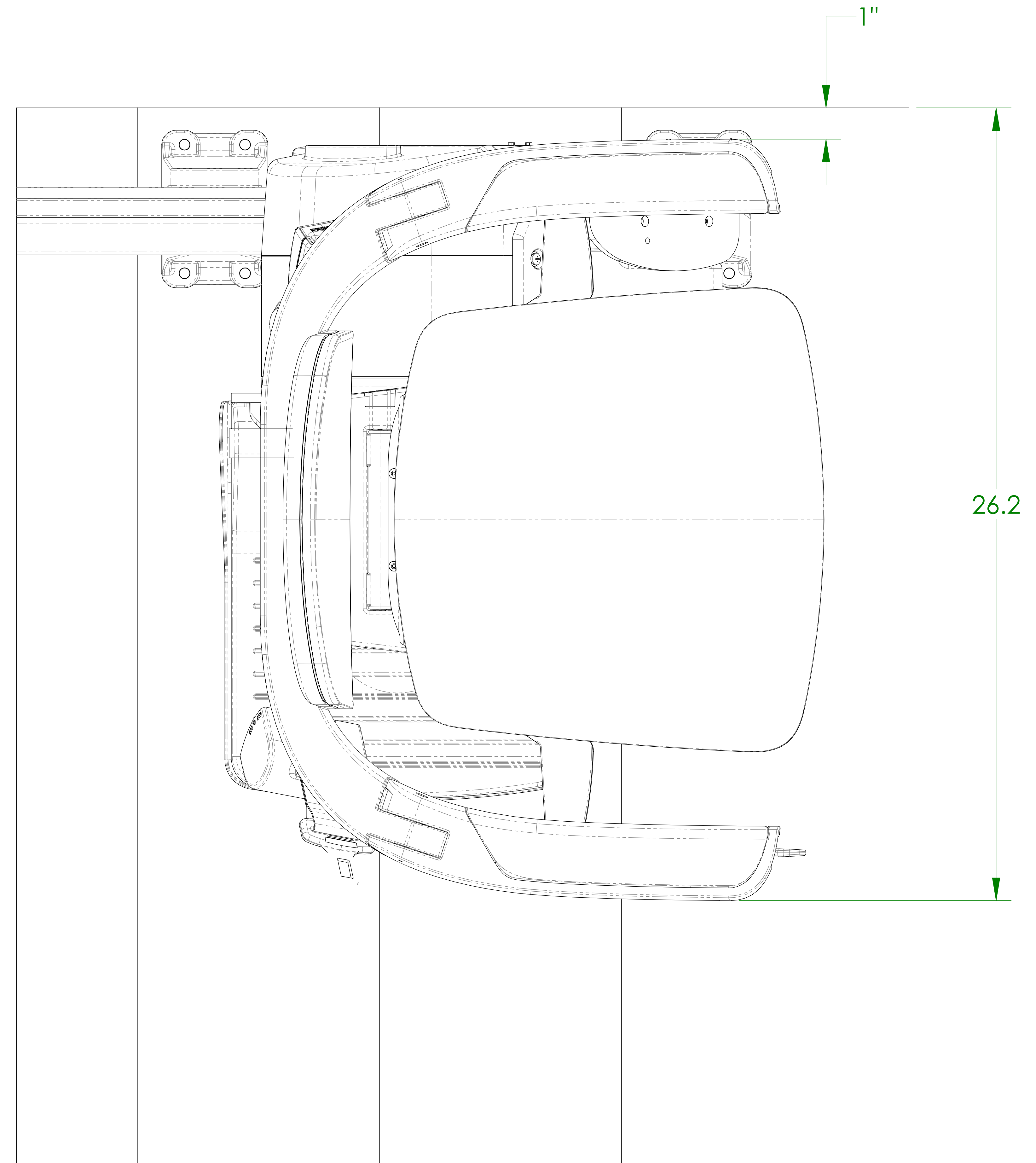
SEAT SWIVELED 90°
